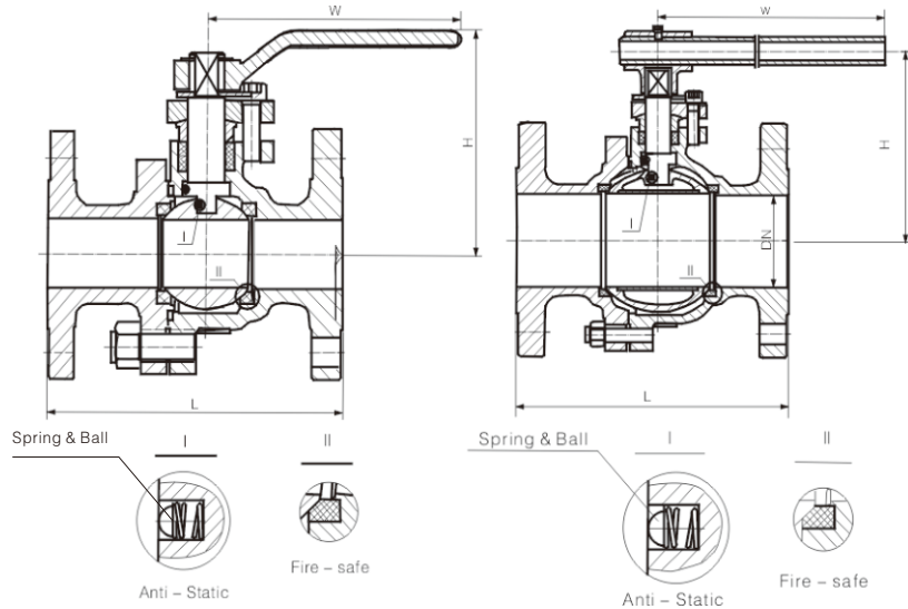
Size main dimensions of Floating Ball Valve
