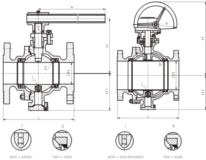
Size main dimensions of Trunnion Ball Valve
